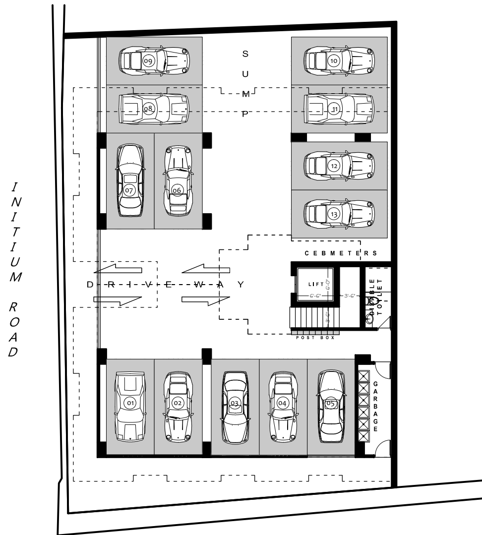
GROUND FLOOR PARKING : 13 NOS.
